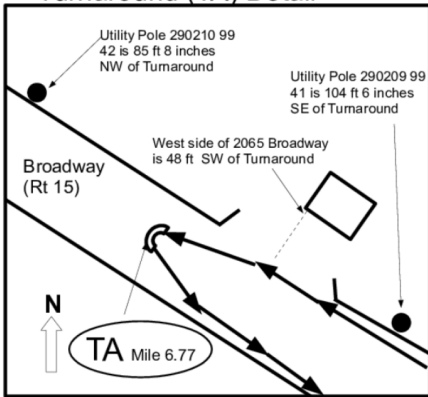
Turnaround (TA) Detail
